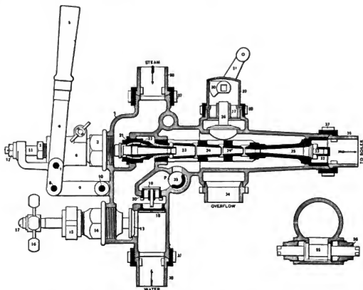
Figs. 3100-3101. Simplex Locomotive Injector. Nathan Manufacturing Co.
